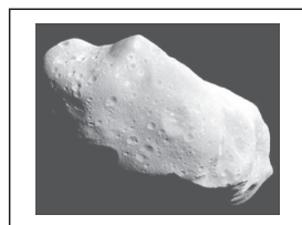
Asteroid
