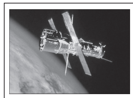
Hubble Telescope
