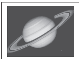
Saturn Planet
