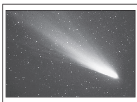
Halley's Comet
